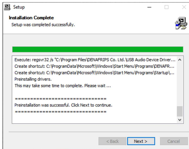
Figure 3. Preinstallation Successful
