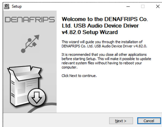
Figure 1. Welcome screen
