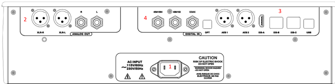
Figure 3. Read Panel
